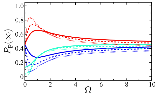
FIG. 3. The asymptotic product population P_P(\infty) of the harmonic potential ( \epsilon = 0 ) as a function of driving frequency \Omega for the \Omega_1 frequency set. The curves are colored with respect to the value of the initial phase shift: \varphi = 0 (blue), \varphi = \pi/2 (cyan), and \varphi = \pi (red). For each value of \varphi , the dependency of the asymptotic population on the friction parameter \gamma is shown by varying the linestyle: \gamma = 0 (solid), \gamma = 1 (dashed), and \gamma = 2 (dotted).
