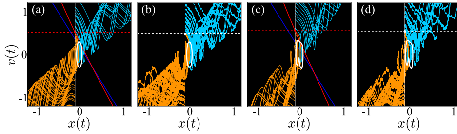
FIG. 2. Phase space plots for a swarm of trajectories following the equations of motion (2) with various driving frequency sets and parameter values: \Omega_1 with \Omega_f = 5 and \epsilon = 1 for (a) \sigma = 0 (noiseless) and (b) \sigma = 0.025 (thermal) driving, \Omega_3 with \Omega_f = 4 and \epsilon = 3 for (c) \sigma = 0 and (d) \sigma = 0.025 . The initial position for every trajectory, x_0 = -0.1 , is shown as a vertical solid white line. Reactive trajectories are colored in cyan and nonreactive trajectories are colored in orange. The TS trajectory \Gamma^\ddagger is shown as a solid white curve. The critical velocity V^\ddagger is indicated by a circle at the intersection of the dashed horizontal line and the line of initial conditions. The solid red curve is the critical curve V_c^\ddagger and the solid blue curve is the harmonic critical curve V_c^\ddagger|_{\epsilon=0} . Parameters for all panels are \gamma = 1 and \varphi = 0 in dimensionless units.
