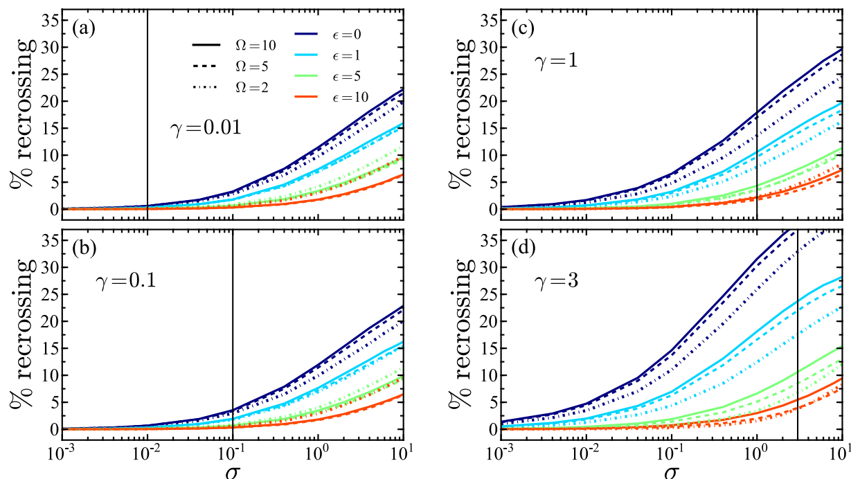
FIG. 6. The percentage of trajectories that recross the moving dividing surface attached to the DTS trajectory as a function of noise strength \sigma with (a) \gamma = 0.01 , (b) \gamma = 0.1 , (c) \gamma = 1 , and (d) \gamma = 3 for single-frequency ( \Omega_1 ) driving and various values of \epsilon and \Omega . The black vertical line (solid) marks the noise strength when the fluctuation-dissipation theorem is obeyed.
