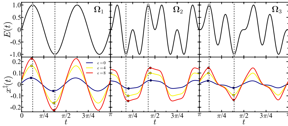
FIG. 1. Functional forms of the periodic driving E(t) for the frequency sets \Omega_1 (left), \Omega_2 (middle), and \Omega_3 (right) with fundamental driving frequency \Omega_f = 4 are shown in the top row. The corresponding TS trajectory for each frequency set and anharmonic parameter values \epsilon \in \{0, 4, 8\} are shown in the bottom row. Various extrema of E(t) are denoted by circles with arguments shown as dashed vertical lines. The corresponding extrema of x^\ddagger(t) are denoted by circles and colored according to the respective \epsilon value. Parameters for all panels are \sigma = 0 , \gamma = 1 , and \varphi = 0 in dimensionless units.
